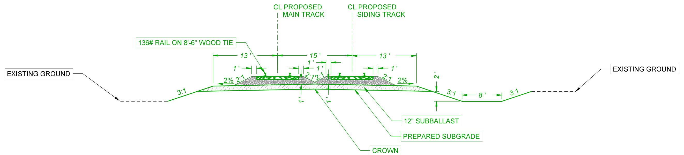
TYPICAL SECTION - SINGLE TRACK w/ SIDING
