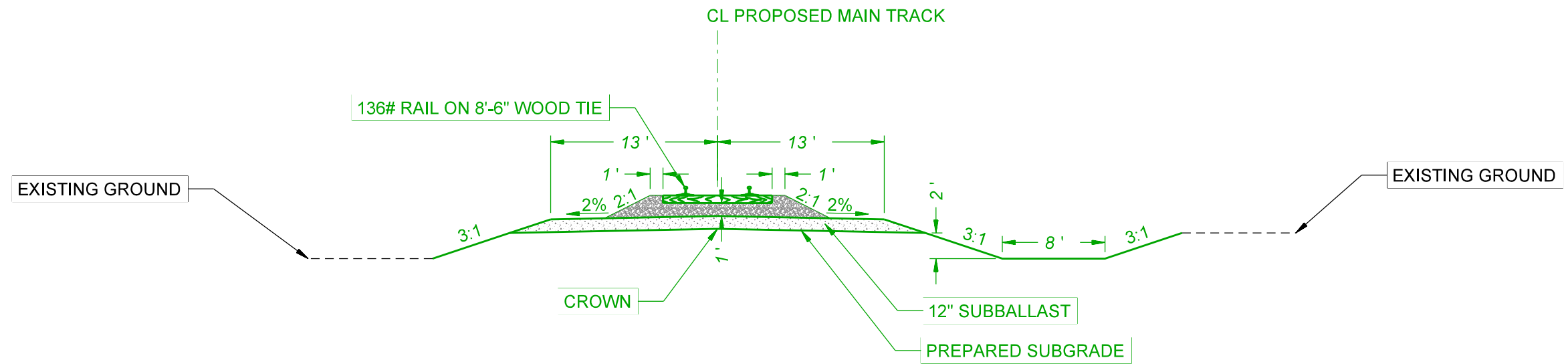
TYPICAL SECTION - SINGLE TRACK
